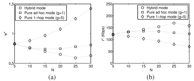
Fig. 7. Performance results in different transmission modes. (a) Minimum scheduling length. (b) Maximum end-to-end throughput.
