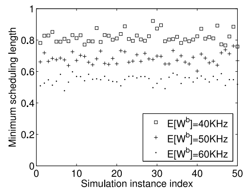
Fig. 12. Minimum scheduling length under different E[W^b] 's for uncertain channel availability.
