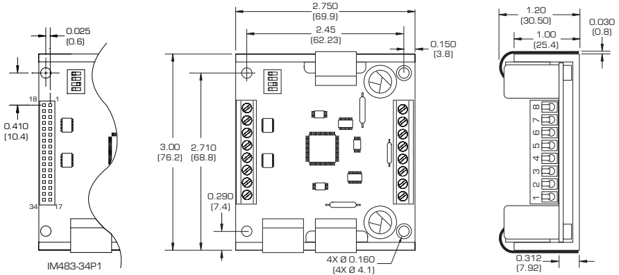
Figure 2.1: IM483 Dimensions
