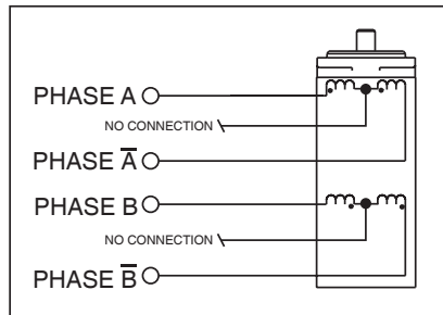
Figure 6.5: 6 Lead Full Coil (Higher Torque) Motor Connections
