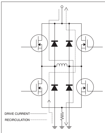
Figure 4.3: Non-Recirculating PWM
