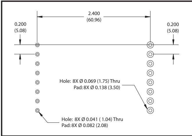
Figure A.7: IM483-8P2 PCB Hole Pattern
