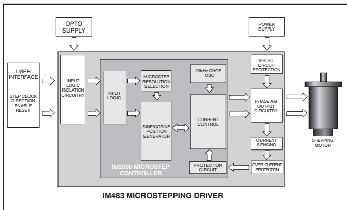
Figure 4.1: IM483 Block Diagram
