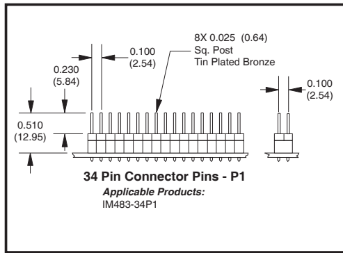
Figure A.1: IM483-34P1 Connector P1 Mechanical Drawing
