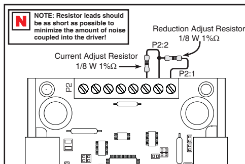
Figure 7.3: Current Reduction Adjust Resistor Placement
