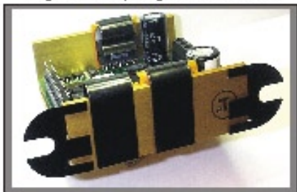
Figure D.2-C: Back view showing clips installed on an IM483
