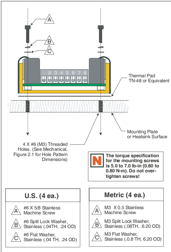
Figure 3.1: Mounting Recommendations
