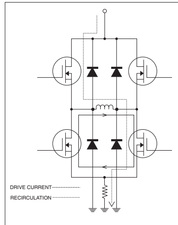
Figure 4.2: Recirculating PWM
