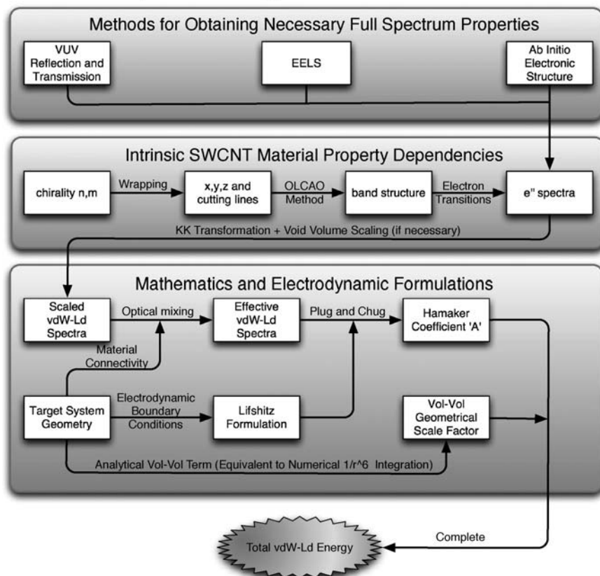
Fig. 1. The complete flow chart of the Lifshitz formulation/framework that is necessary for calculating and understanding the physical origin of the chirality-dependent Hamaker coefficients and vdW–Ld total energies of SWCNT systems.
