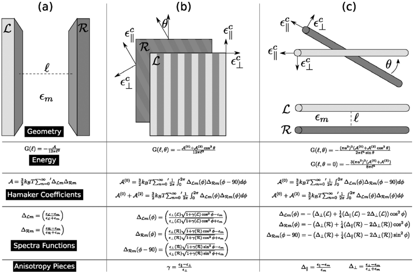
Fig. 7. The 3 different systems of comparison. (a) Isotropic semi-infinite half spaces (b) Anisotropic semi-infinite half spaces (c) Anisotropic solid cylinders. The energy \mathcal{G} is in units of per nm^2 of substrate area in a) and b) versus per nm of cylinder in c).
