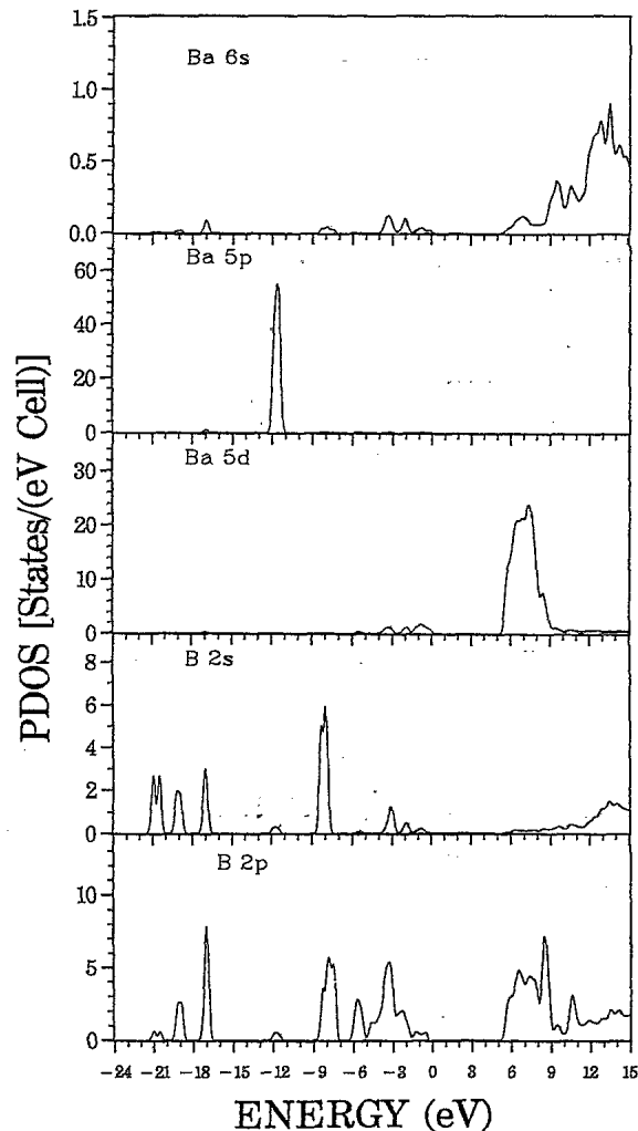
FIG. 3. Orbital-resolved partial DOS of Ba and B in \beta -BaB 2 O 4 .
