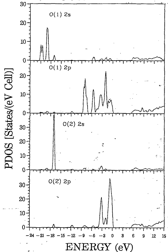
FIG. 4. Orbital-resolved partial DOS of O(1) and O(2) in \beta -BaB 2 O 4 .
