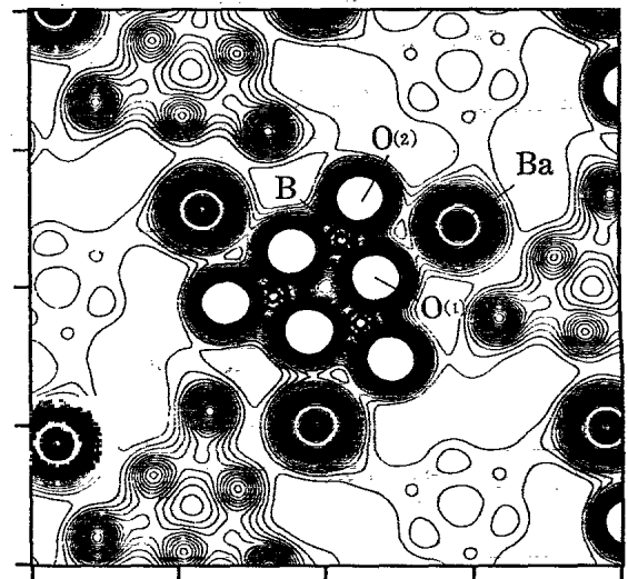
FIG. 5. Charge-density distribution in \beta -BaB 2 O 4 on the [001] plane containing a (B_3O_6)^{-3} unit (at the center). The other charges are from ions in the planes adjacent to it. The contour lines are from 0.01 to 0.25 by 0.005 all in units of electrons/(a.u.) -3 .
