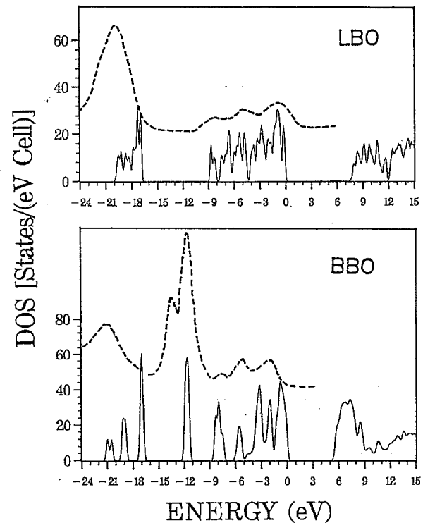
FIG. 2. Total DOS of (a) LBO and (b) BBO. The dashed lines are the experimental XPS data from Ref. 8.
