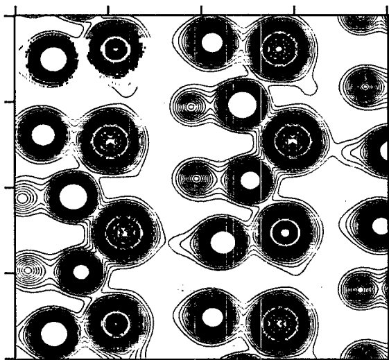
FIG. 7. Charge-density distribution in \beta -BaB 2 O 4 in a plane parallel to the c axis. The contour units are the same as Fig. 5. Note that only five of the Ba ions in this diagram are strictly in the plane.
