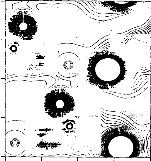
FIG. 9. Charge-density distribution in \text{LiB}_3\text{O}_5 in the a - c plane with y=0 .
